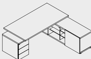
MIT1KD 2497 | 2080 | 740 98 3/8" | 82" | 29 1/8"
