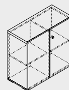
MIT21 916 | 418 | 879 36 1/8" | 16 1/2" | 34 5/8"
