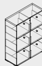
MIT22 980 | 418 | 1280 38 5/8" | 16 1/2" | 50 1/2"
