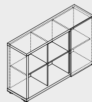
MIT18 1400 | 422 | 879 55 1/8" | 16 5/8" | 34 5/8"
