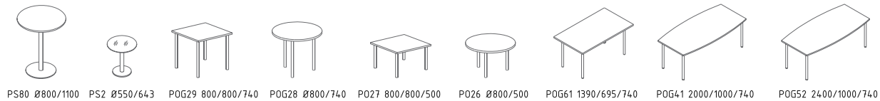
PS80 Ø800/1100 PS2 Ø550/643 POG29 800/800/740 POG28 Ø800/740 POG2 800/800/500 POG26 Ø800/500 POG61 1390/695/740 POG41 2000/1000/740 POG52 2400/1000/740
